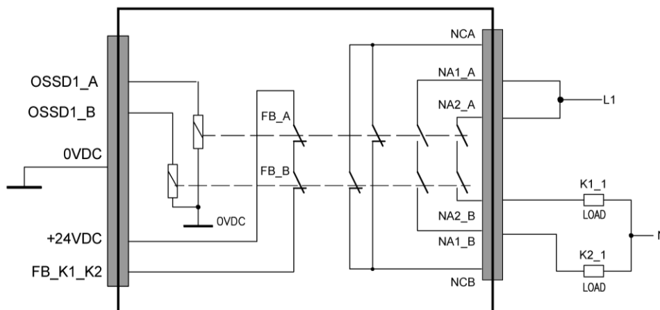
Figure 6 – M SG BOX connection sample
