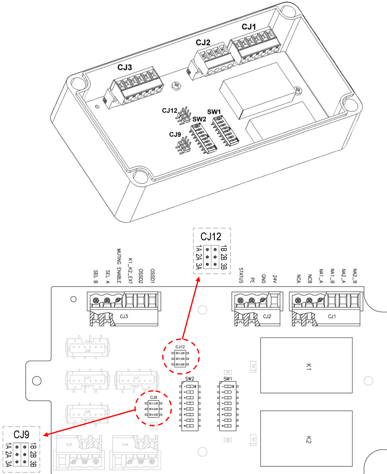
Figure 5 – Main board
