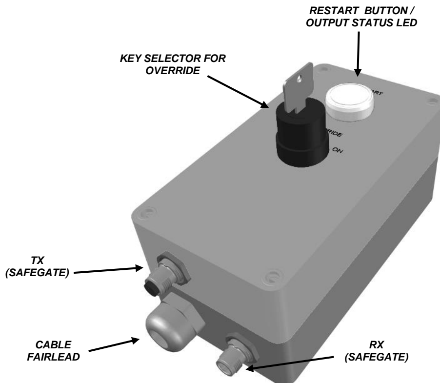
Figure 4 - M SG BOX – Connections and signals
